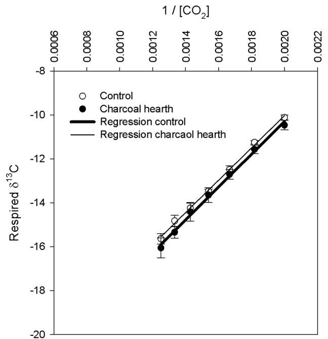
Figure 3. Keeling plots measured by CRDS showing the \delta^{13}C of respired CO 2 fluxes versus the reciprocal of CO 2 concentration for control and charcoal hearth incubated soils ( \delta^{13}C_{CONTROL} = 7353 * [CO_2]^{-1} - 24.8 , R^2 = 0.99 ; \delta^{13}C_{CHARCOAL HEARTH} = 7467 * [CO_2]^{-1} - 25.2 , R^2 = 0.99 ). Horizontal and vertical bars indicate standard deviations (n=3). doi:10.1371/journal.pone.0091114.g003
